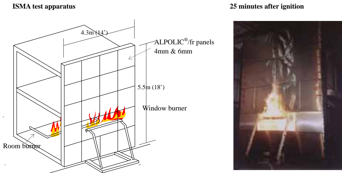
Fig. 2-5 Intermediate-scale Multistory Apparatus
