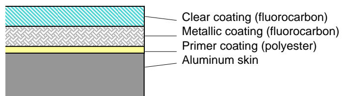
Fig. 2-9 3-coat, 3-bake system for Metallic Colors
