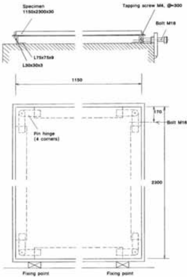
Fig. 2-12 Test of shearing force for earthquakes
